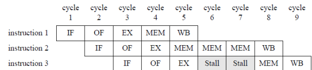
Figure 3. 5-Stage pipelining timing diagram
