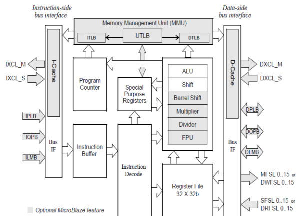
Figure 2. Proposed architecture of multiprocessor architecture.
